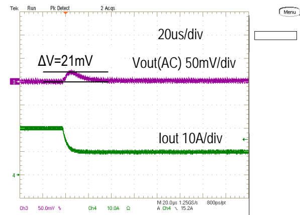
Step Load Transient Response (Vin=5.0V, Vout=1.0V, Cloud=660uF, Iout=20A to 10A, 2.5A/us)
