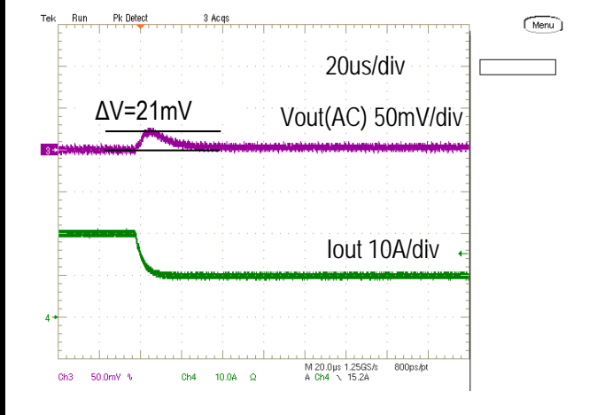
Step Load Transient Response (Vin=5.0V, Vout=0.7V, Load=660uF, Iout=20A to 10A, 2.5A/us)
