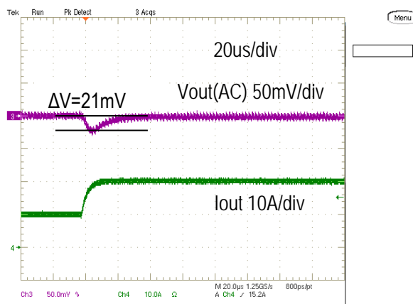
Step Load Transient Response (Vin=5.0V, Vout=1.0V, Cloud=660uF, Iout=10A to 20A, 2.5A/us)
