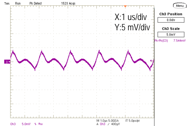
Output Ripple and Noise (Vin=5.0V, Vout=1.0V, Iout=20A, Load=660uF, ScopeBW=20MHz)
