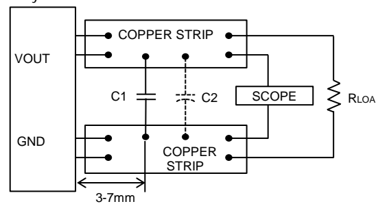
C1=220uF x 3 CERAMIC C2=OPEN
