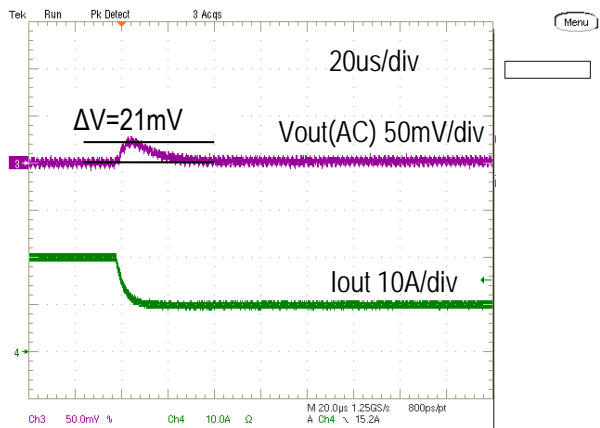
Step Load Transient Response (Vin=5.0V, Vout=1.8V, Load=660uF, Iout=20A to 10A, 2.5A/us)
