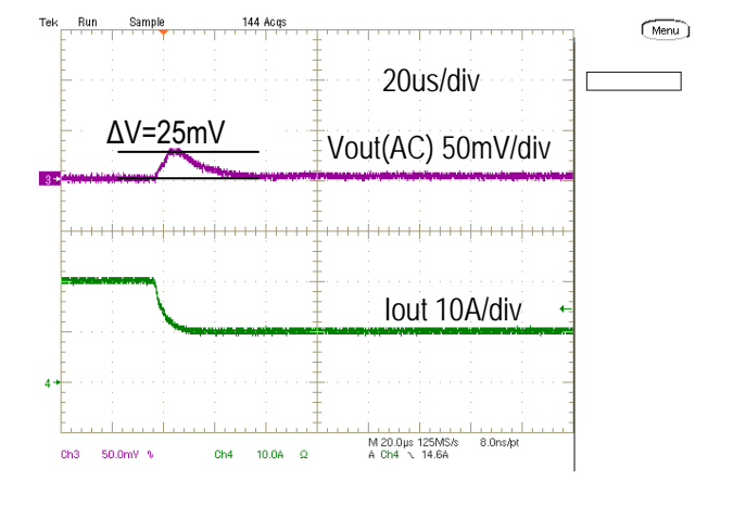
Step Load Transient Response (Vin=12.0V, Vout=0.7V, Cload=660uF, Iout=20A to 10A, 2.5A/us)
