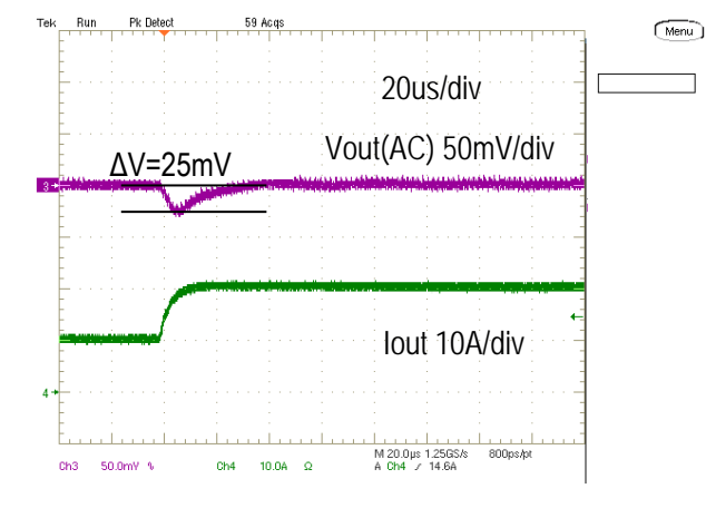
Step Load Transient Response (Vin=12.0V, Vout=1.8V, Cload=660uF, Iout=10A to 20A, 2.5A/us)
