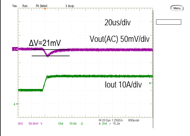
Step Load Transient Response (Vin=5.0V, Vout=0.7V, Load=660uF, Iout=10A to 20A, 2.5A/us)
