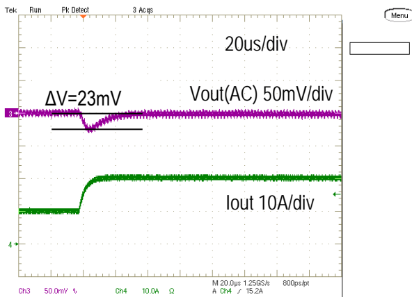
Step Load Transient Response (Vin=5.0V, Vout=1.8V, Load=660uF, Iout=10A to 20A, 2.5A/us)
