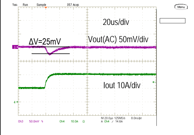
Step Load Transient Response (Vin=12.0V, Vout=1.0V, Cload=660uF, Iout=10A to 20A, 2.5A/us)
