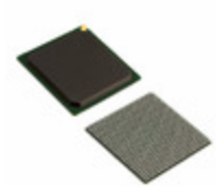
XC7A75T-3FGG676E AMD IC FPGA 300 I/O 676FBGA
