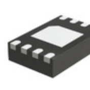
24AA025T-I/MNY Microchip Technology IC EEPROM 2KBIT I2C 400KHZ 8TDFN
