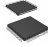
EPM7064AETC100-7 Intel IC CPLD 64MC 7.5NS 100TQFP
