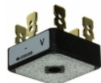
VS-26MT60
