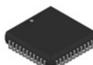
EPM7032AELC44-4 Altera IC CPLD 32MC 4.5NS 44PLCC
