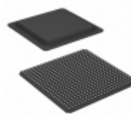
XC7A75T-1FGG484C AMD IC FPGA 285 I/O 484FBGA
