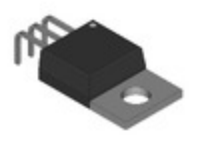
BTA12-800CW3G onsemi SNUBBERLESS TRIAC, 800V, 12A, TO
