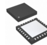
PIC16LF1786-I/ML Microchip Technology IC MCU 8BIT 14KB FLASH 28QFN
