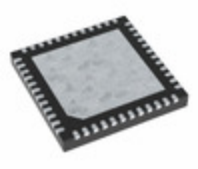
KSZ9031RNXCC Microchip Technology IC TRANSCEIVER FULL 4/4 48QFN
